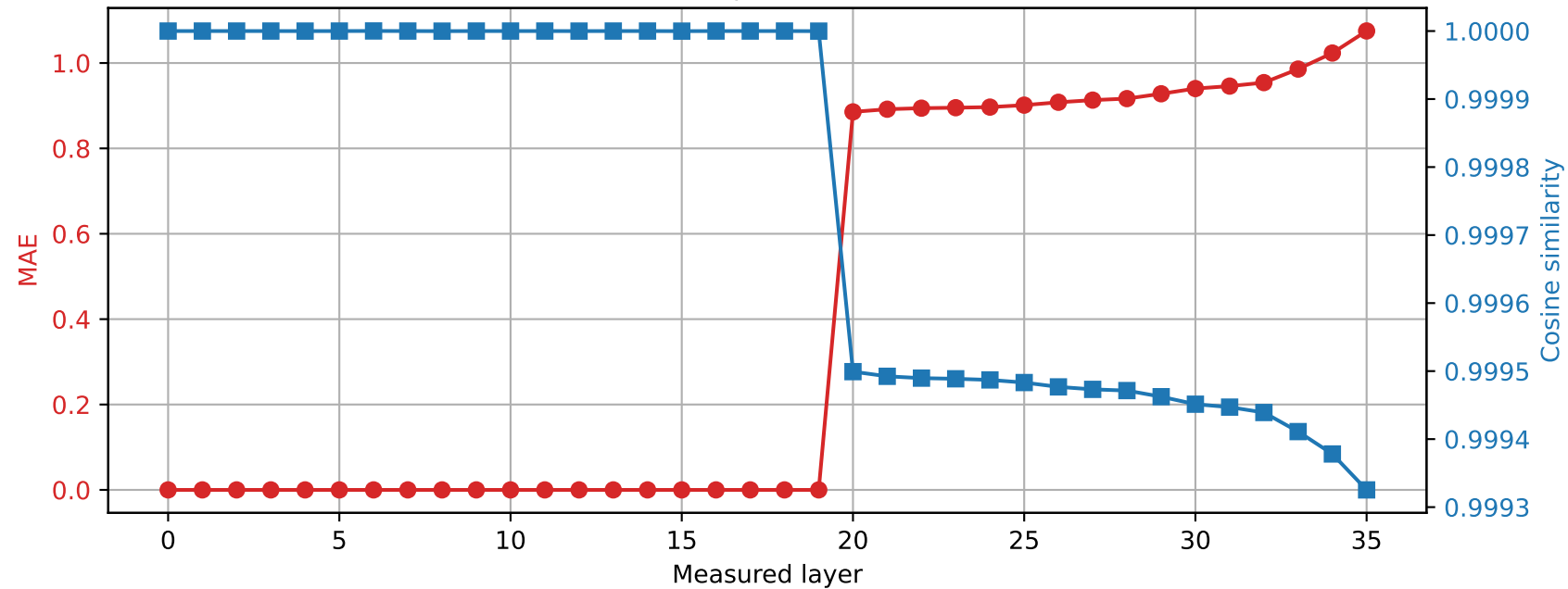
Qwen2.5-3B | Prompt 2 Spared layer 19 | Hybrid vs quantized
