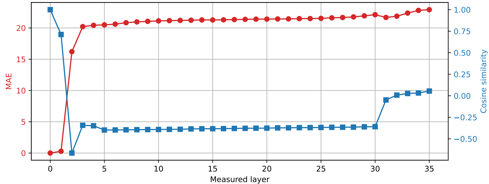
Qwen2.5-3B | Prompt 2 Spared layer 34 | Hybrid vs unquantized
