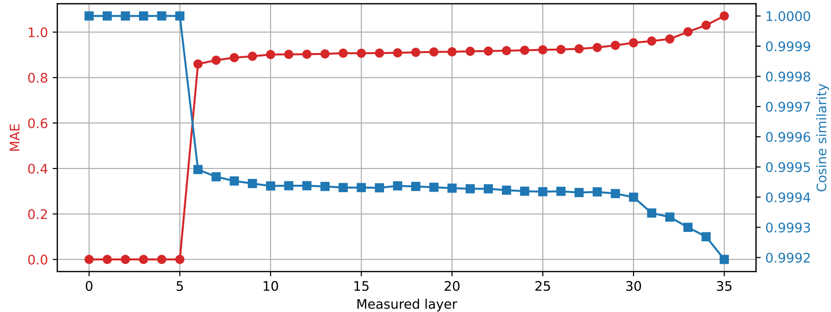
Qwen2.5-3B | Prompt 3 Spared layer 5 | Hybrid vs quantized
