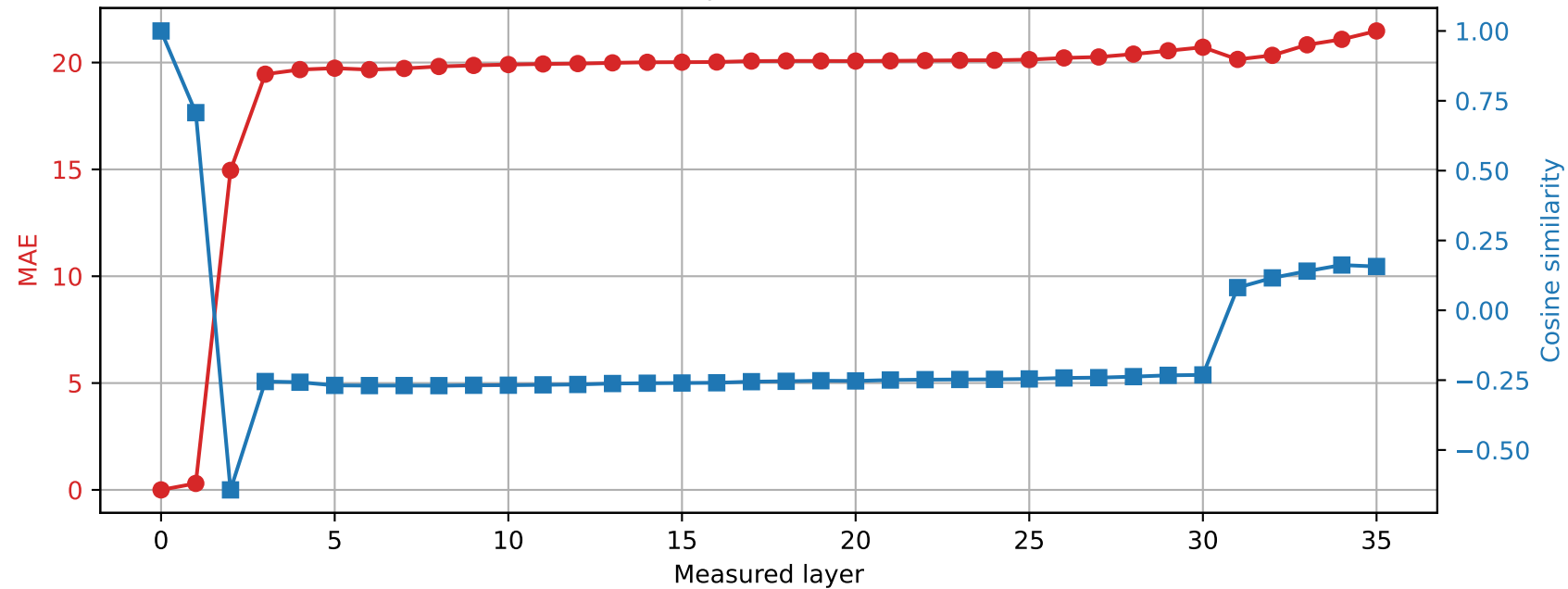
Qwen2.5-3B | Prompt 3 Spared layer 5 | Hybrid vs unquantized
