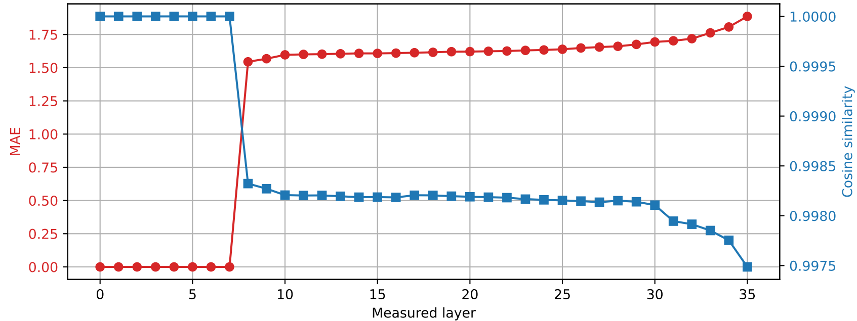
Qwen2.5-3B | Prompt 3 Spared layer 7 | Hybrid vs quantized
