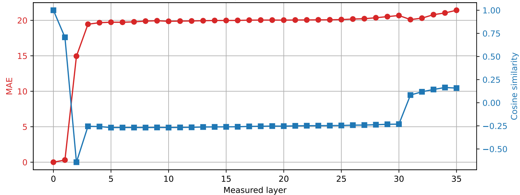
Qwen2.5-3B | Prompt 3 Spared layer 9 | Hybrid vs unquantized
