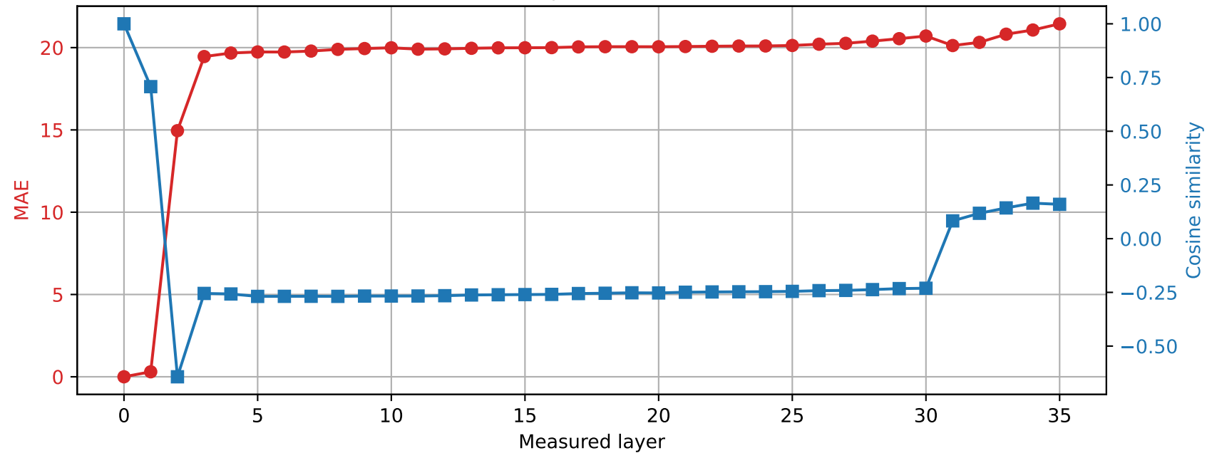
Qwen2.5-3B | Prompt 3 Spared layer 10 | Hybrid vs unquantized
