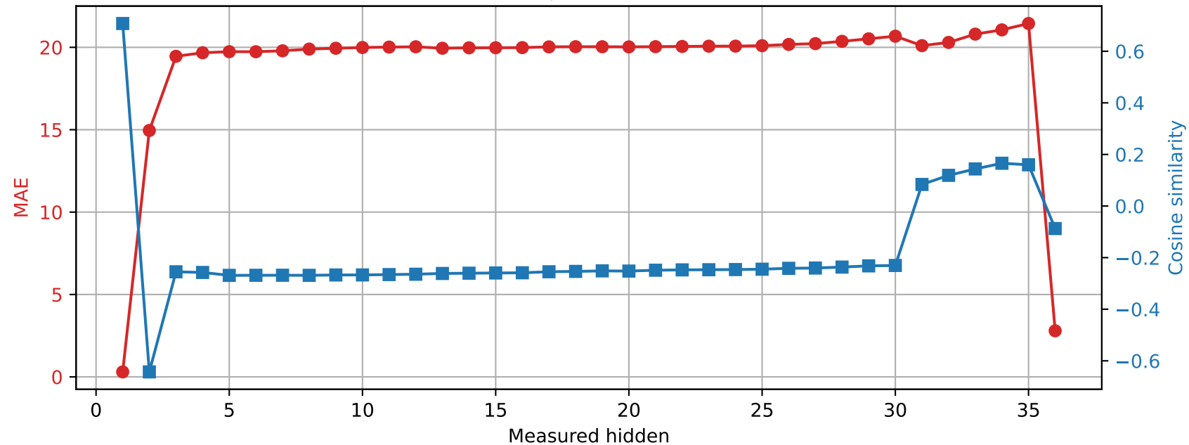
Qwen2.5-3B | Prompt 3 Spared layer 12 | Unquantized vs hybrid
