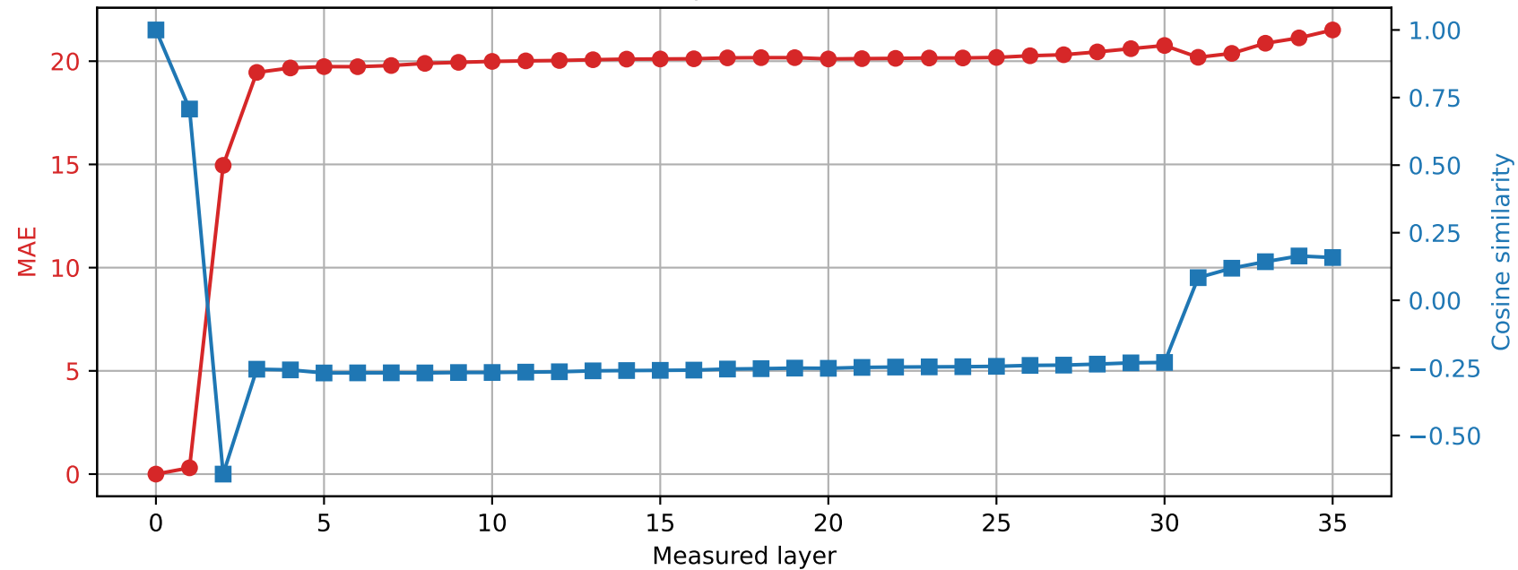
Qwen2.5-3B | Prompt 3 Spared layer 19 | Hybrid vs unquantized
