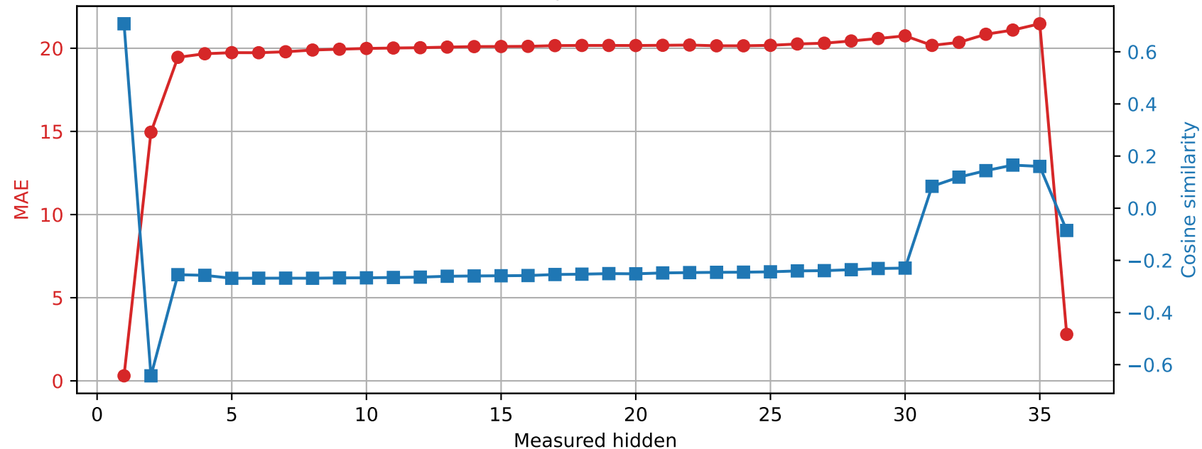
Qwen2.5-3B | Prompt 3 Spared layer 22 | Unquantized vs hybrid
