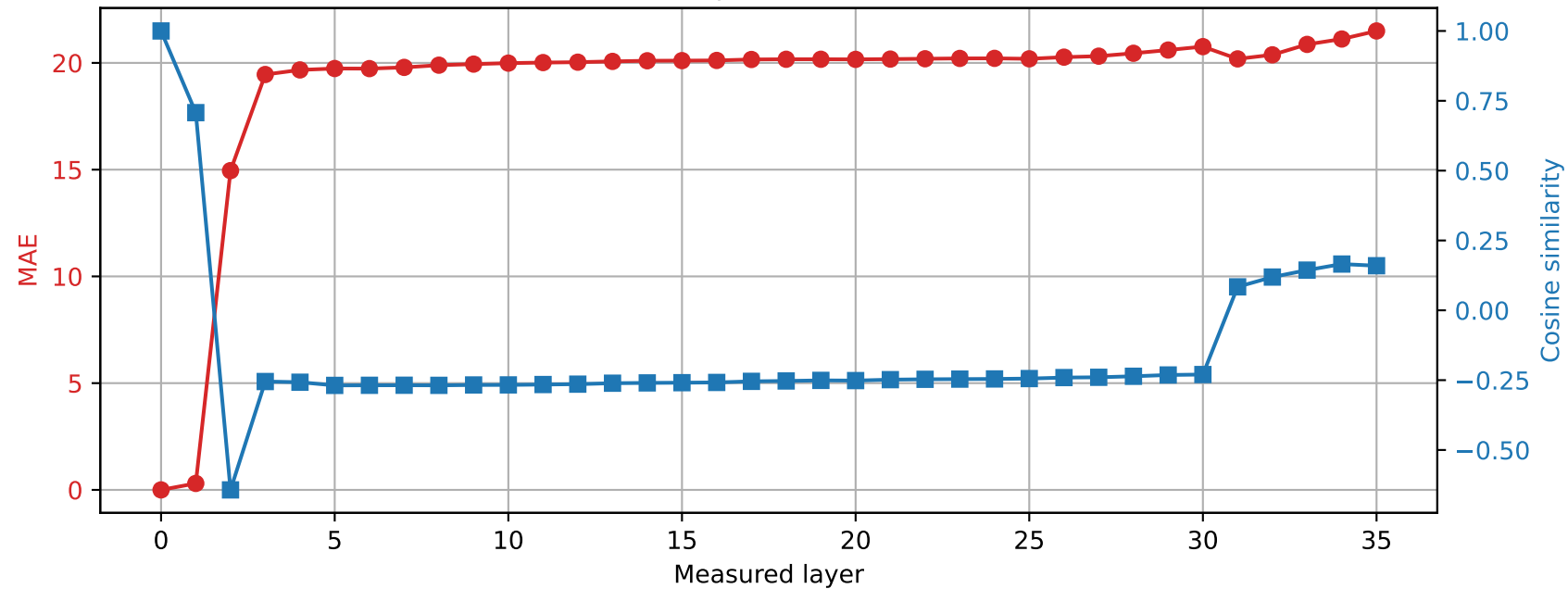
Qwen2.5-3B | Prompt 3 Spared layer 24 | Hybrid vs unquantized
