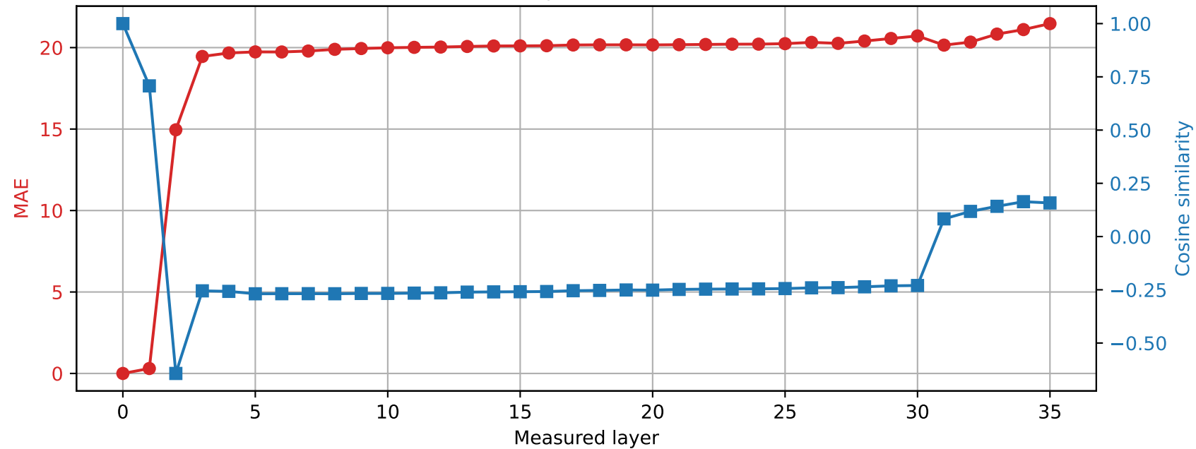
Qwen2.5-3B | Prompt 3 Spared layer 26 | Hybrid vs unquantized
