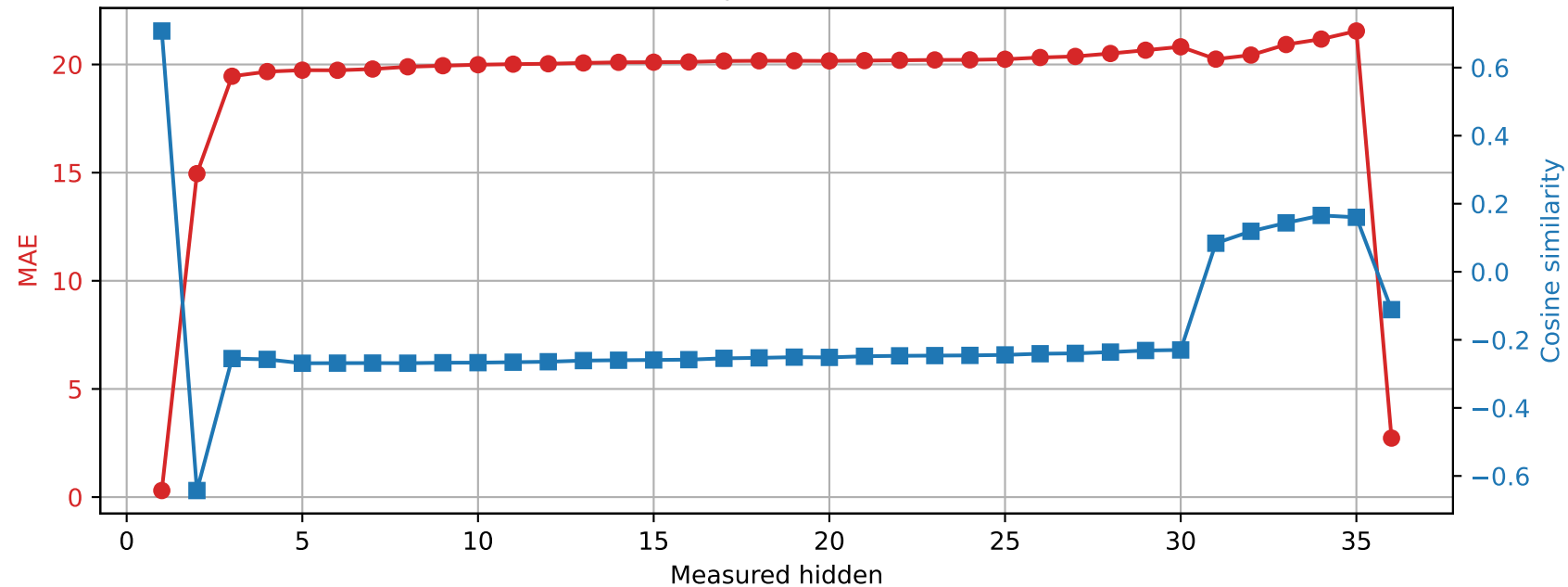
Qwen2.5-3B | Prompt 3 Spared layer 35 | Unquantized vs hybrid
