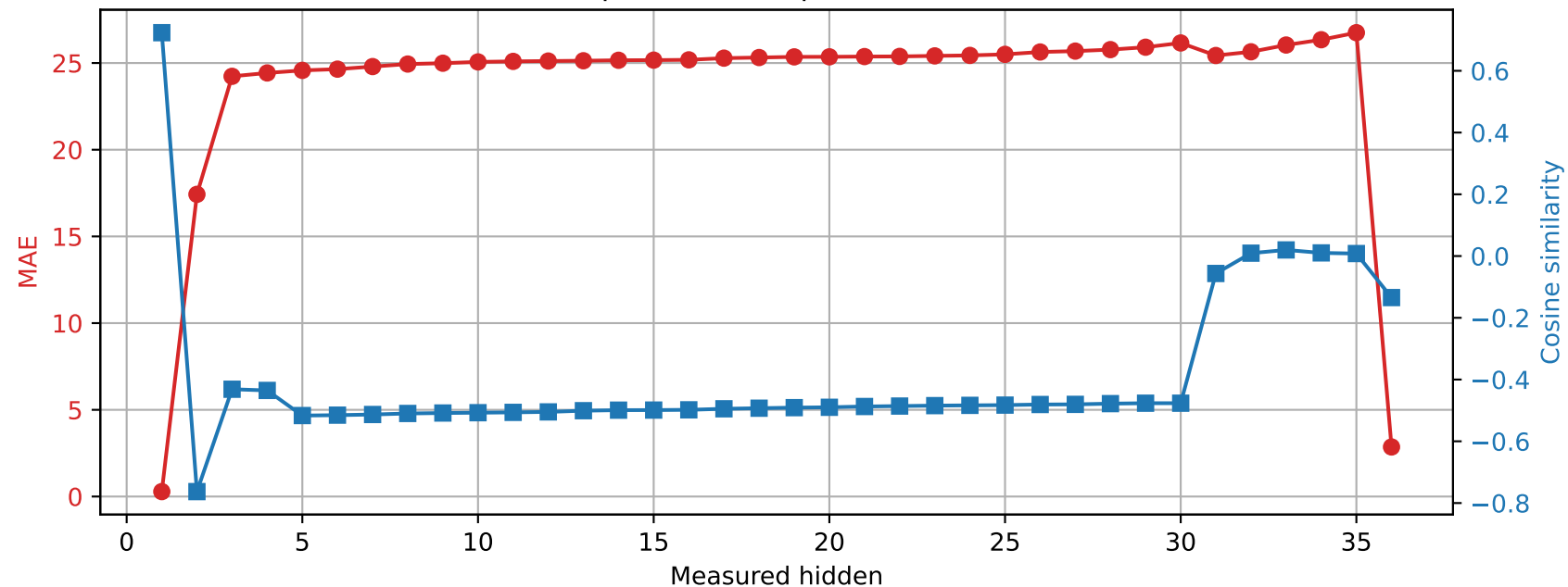
Qwen2.5-3B | Prompt 4 Unquantized vs quantized int4
