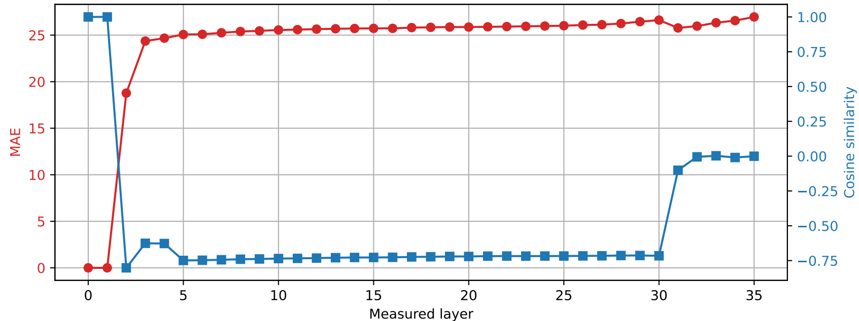
Qwen2.5-3B | Prompt 4 Spared layer 0 | Hybrid vs unquantized
