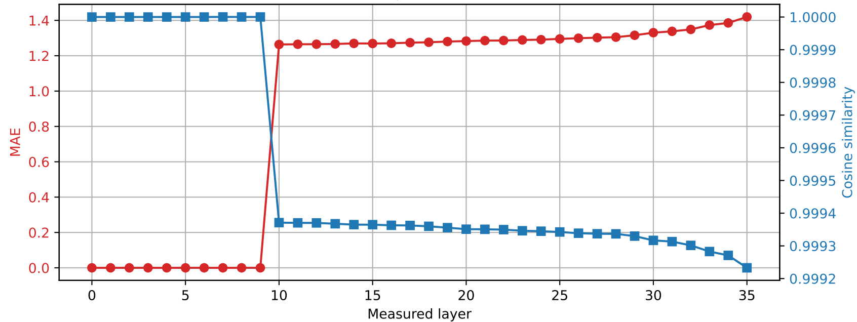
Qwen2.5-3B | Prompt 4 Spared layer 9 | Hybrid vs quantized
