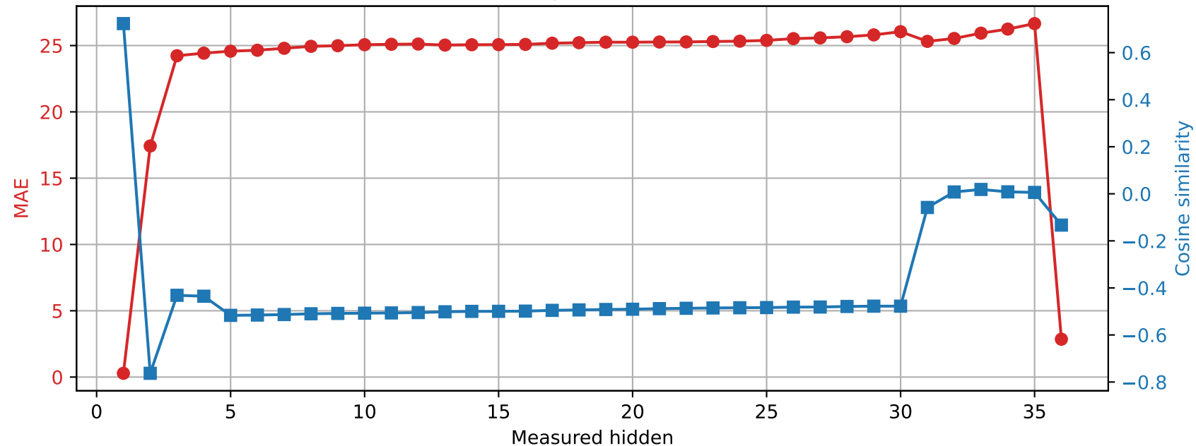
Qwen2.5-3B | Prompt 4 Spared layer 12 | Unquantized vs hybrid
