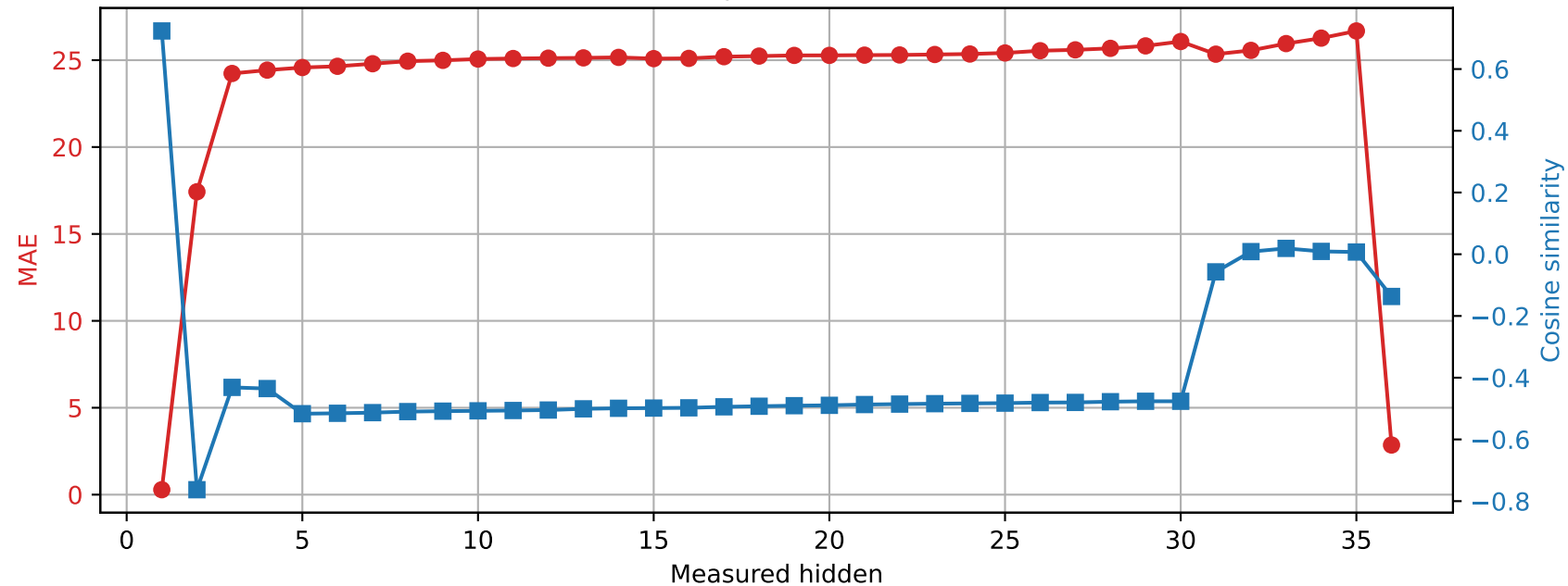
Qwen2.5-3B | Prompt 4 Spared layer 14 | Unquantized vs hybrid
