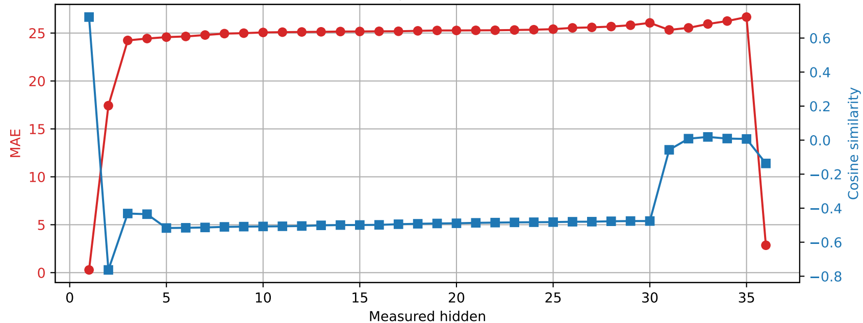
Qwen2.5-3B | Prompt 4 Spared layer 16 | Unquantized vs hybrid
