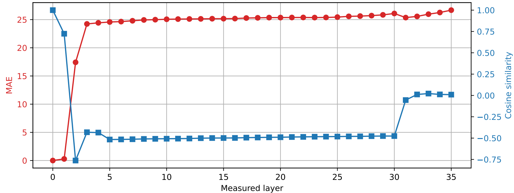
Qwen2.5-3B | Prompt 4 Spared layer 22 | Hybrid vs unquantized
