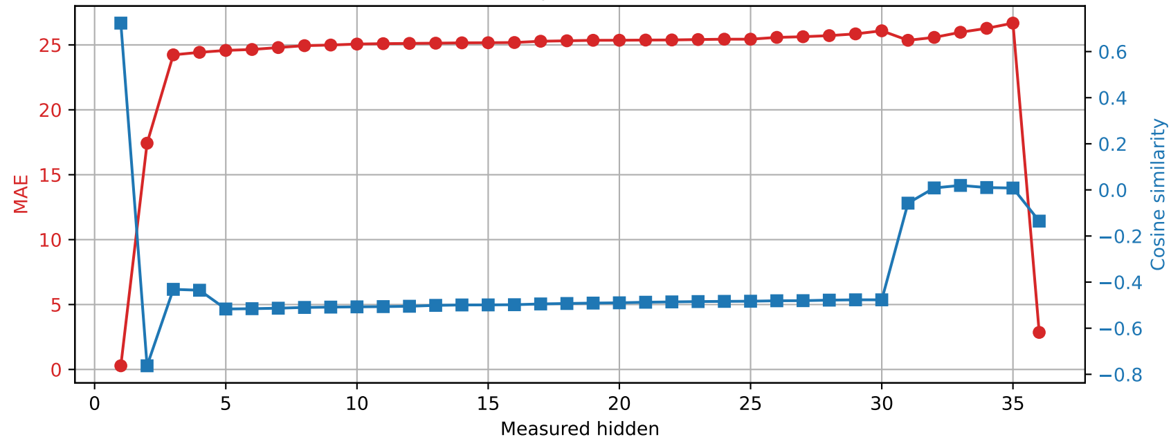
Qwen2.5-3B | Prompt 4 Spared layer 24 | Unquantized vs hybrid
