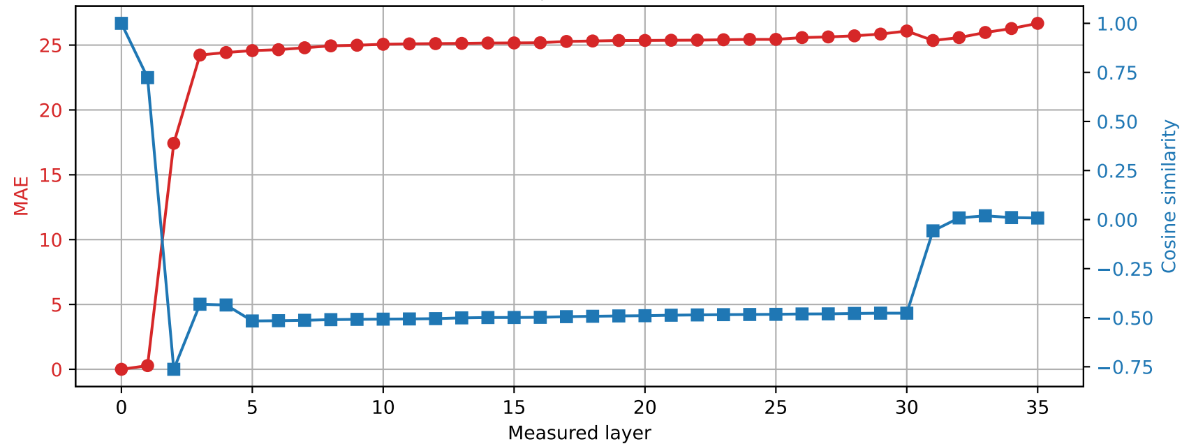
Qwen2.5-3B | Prompt 4 Spared layer 24 | Hybrid vs unquantized
