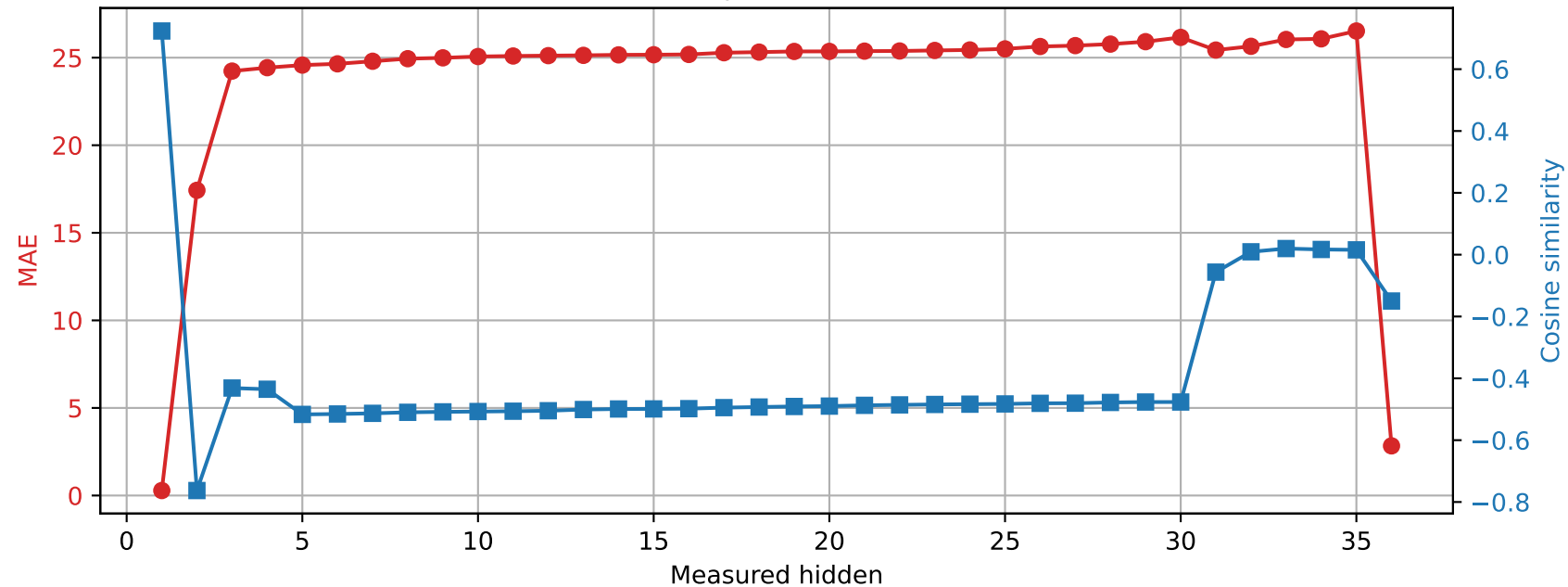
Qwen2.5-3B | Prompt 4 Spared layer 33 | Unquantized vs hybrid
