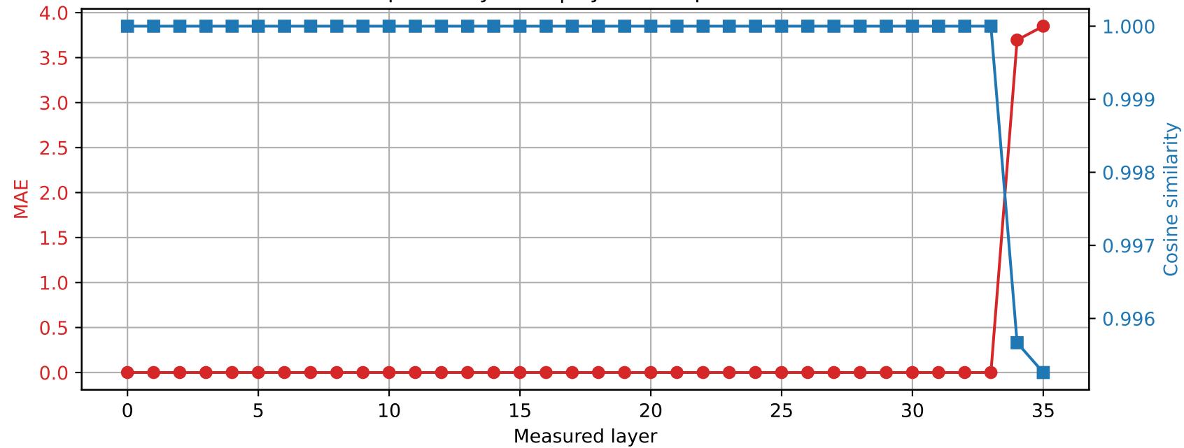
Qwen2.5-3B | Prompt 4 Spared layer 33 | Hybrid vs quantized
