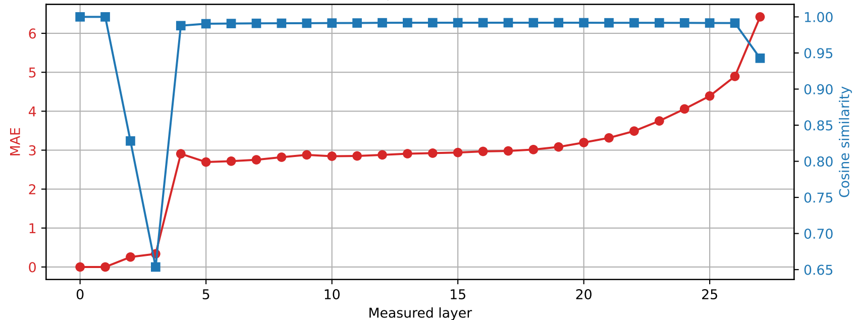
Qwen2.5-7B-Instruct | Prompt 0 Spared layer 0 | Hybrid vs unquantized
