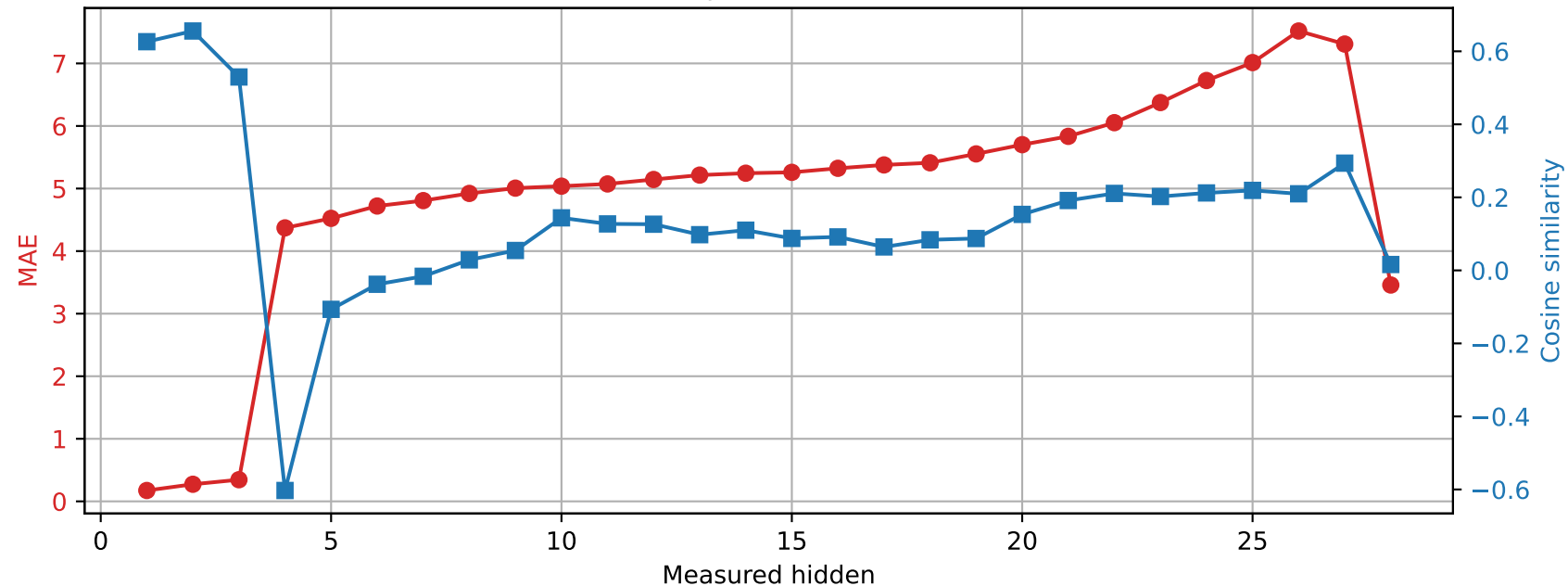
Qwen2.5-7B-Instruct | Prompt 0 Spared layer 1 | Unquantized vs hybrid
