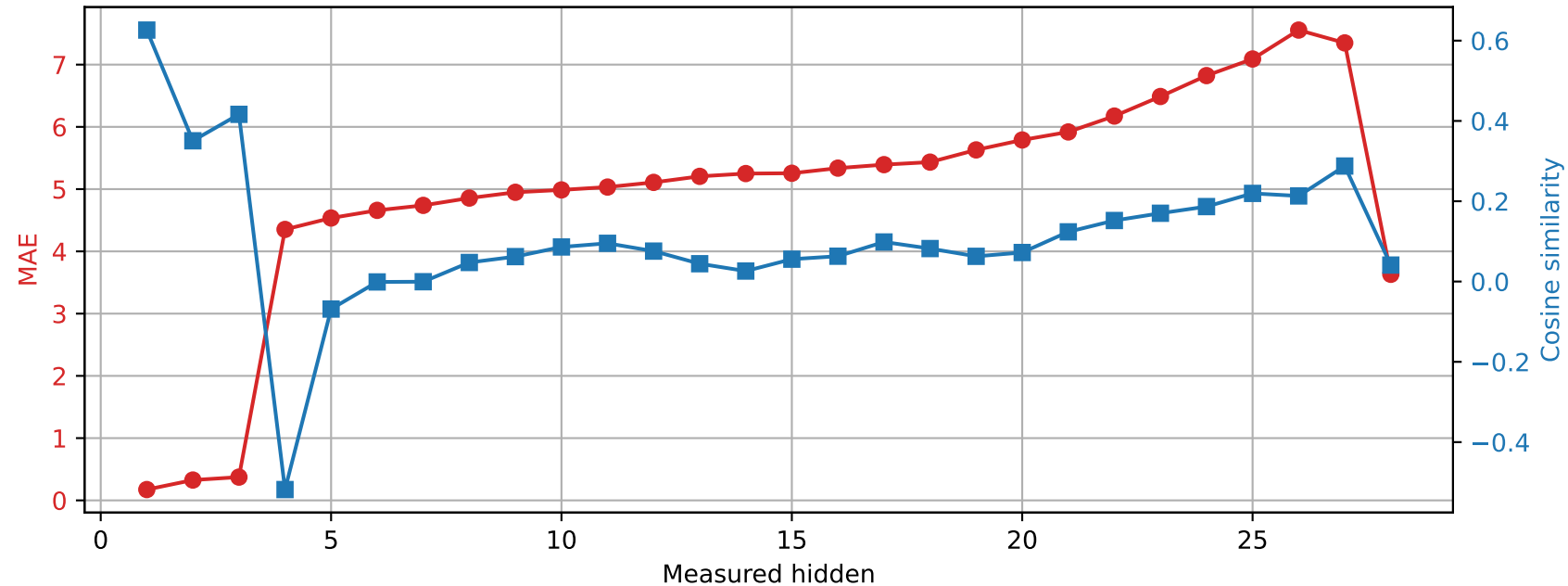
Qwen2.5-7B-Instruct | Prompt 0 Spared layer 2 | Unquantized vs hybrid
