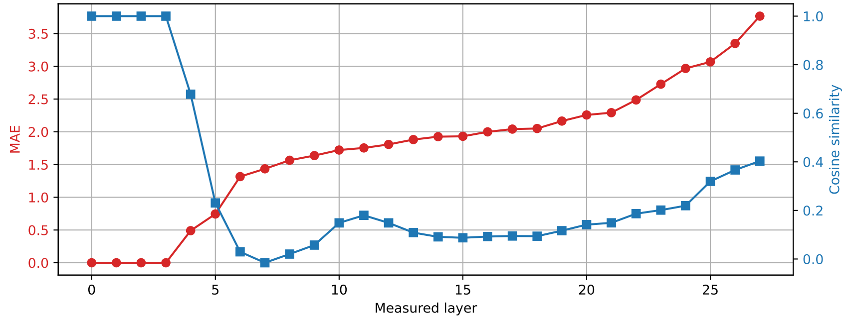
Qwen2.5-7B-Instruct | Prompt 0 Spared layer 3 | Hybrid vs quantized
