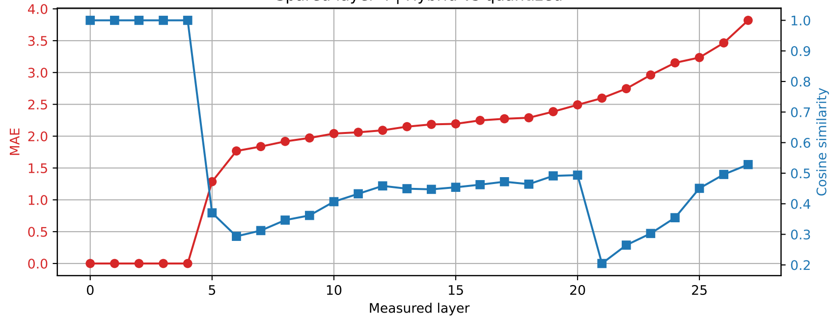
Qwen2.5-7B-Instruct | Prompt 0 Spared layer 4 | Hybrid vs quantized
