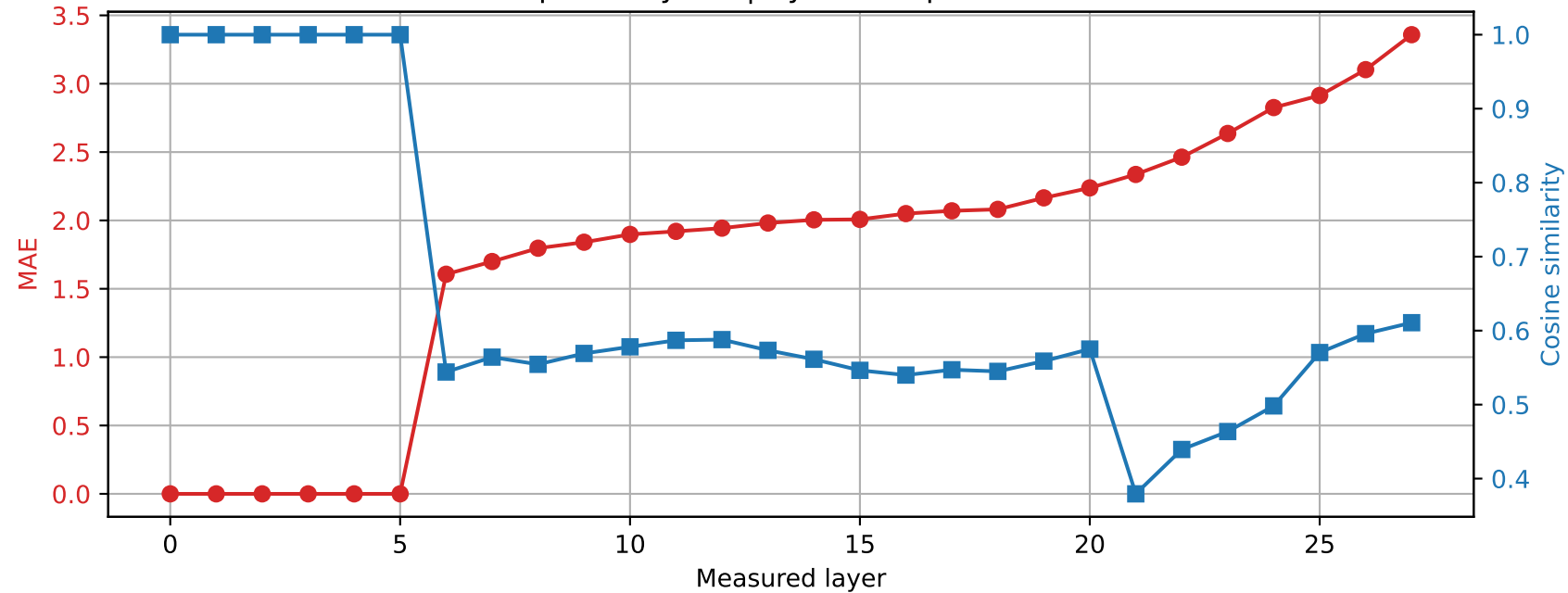
Qwen2.5-7B-Instruct | Prompt 0 Spared layer 5 | Hybrid vs quantized
