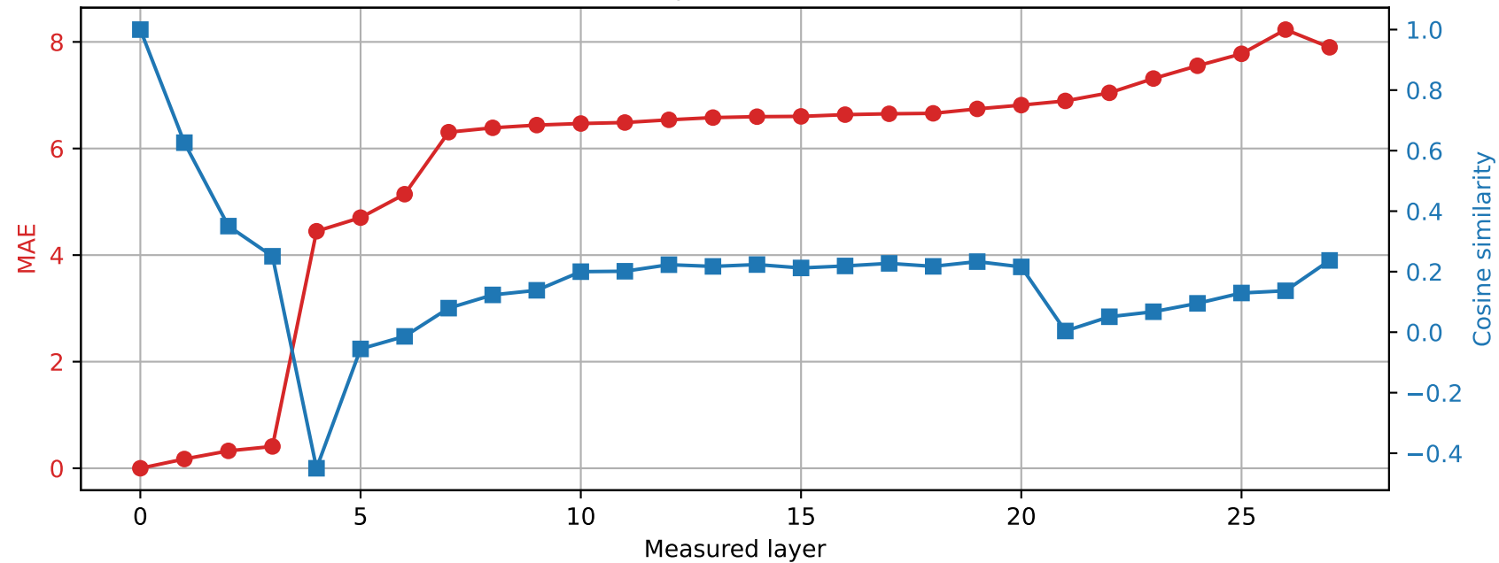
Qwen2.5-7B-Instruct | Prompt 0 Spared layer 6 | Hybrid vs unquantized
