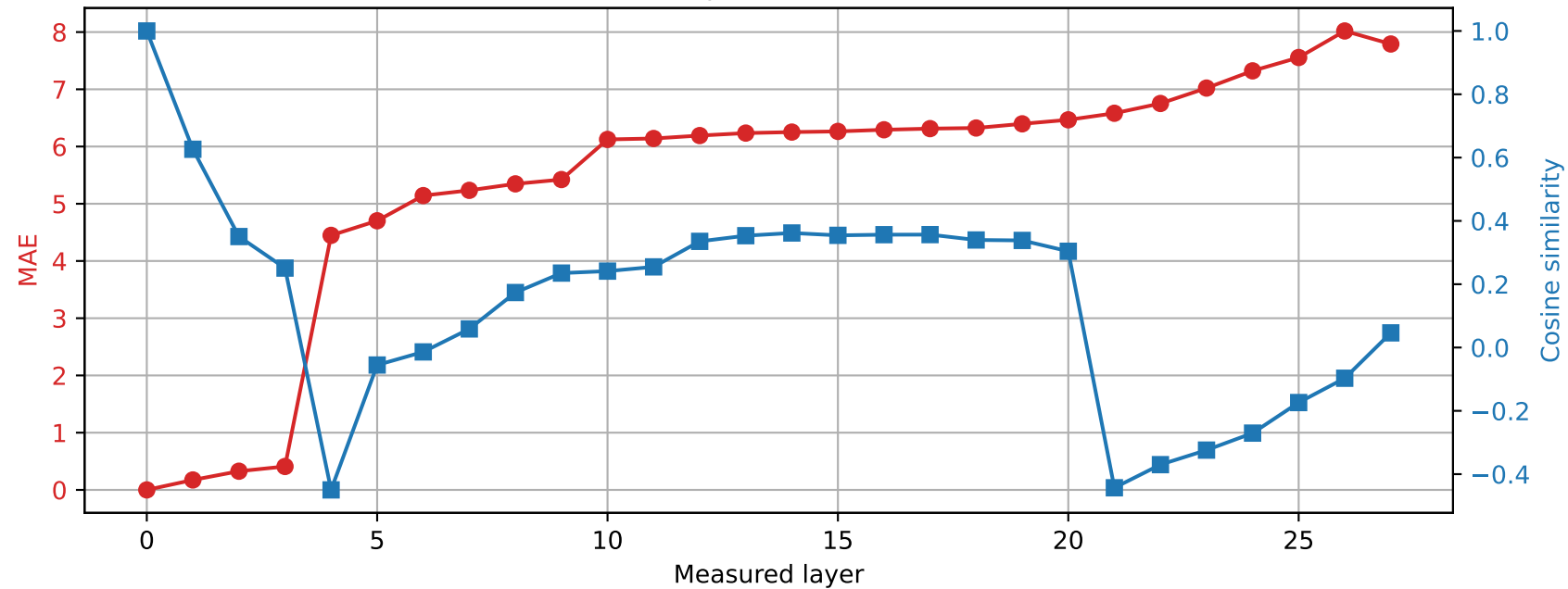
Qwen2.5-7B-Instruct | Prompt 0 Spared layer 9 | Hybrid vs unquantized
