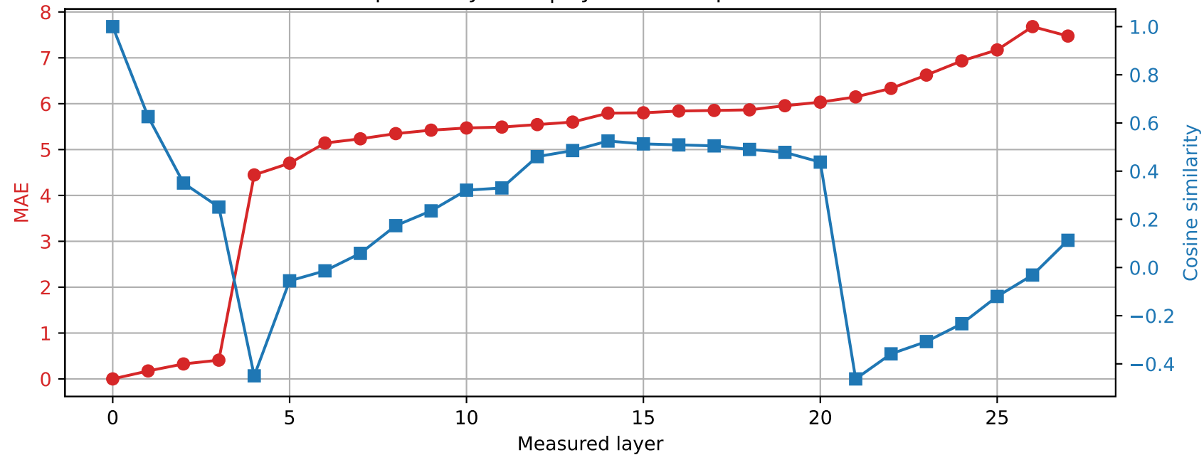
Qwen2.5-7B-Instruct | Prompt 0 Spared layer 13 | Hybrid vs unquantized
