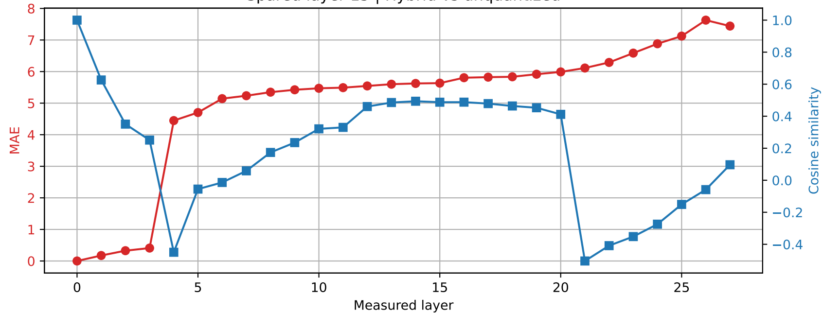
Qwen2.5-7B-Instruct | Prompt 0 Spared layer 15 | Hybrid vs unquantized
