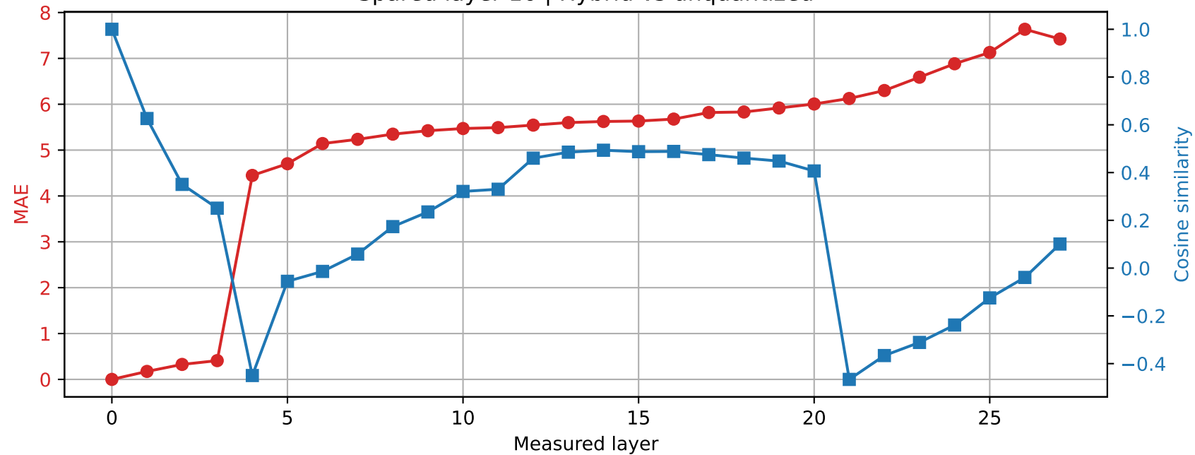
Qwen2.5-7B-Instruct | Prompt 0 Spared layer 16 | Hybrid vs unquantized
