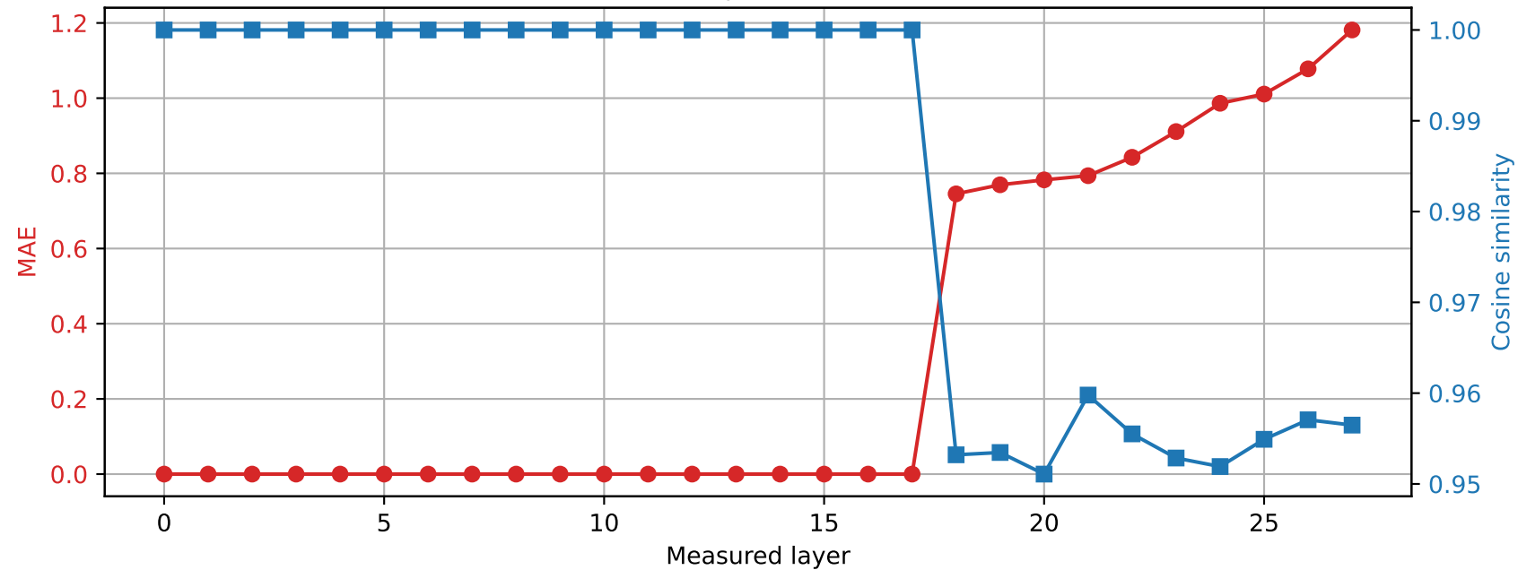
Qwen2.5-7B-Instruct | Prompt 0 Spared layer 17 | Hybrid vs quantized
