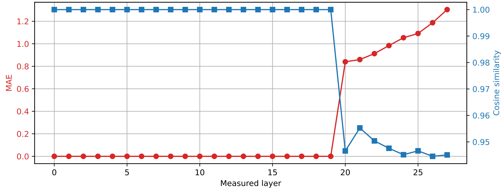
Qwen2.5-7B-Instruct | Prompt 0 Spared layer 19 | Hybrid vs quantized
