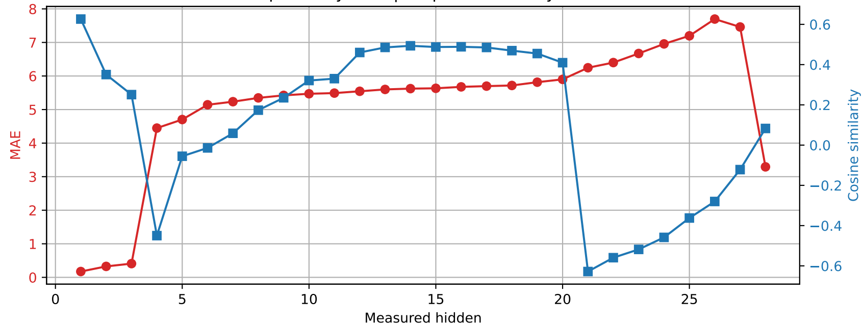
Qwen2.5-7B-Instruct | Prompt 0 Spared layer 20 | Unquantized vs hybrid
