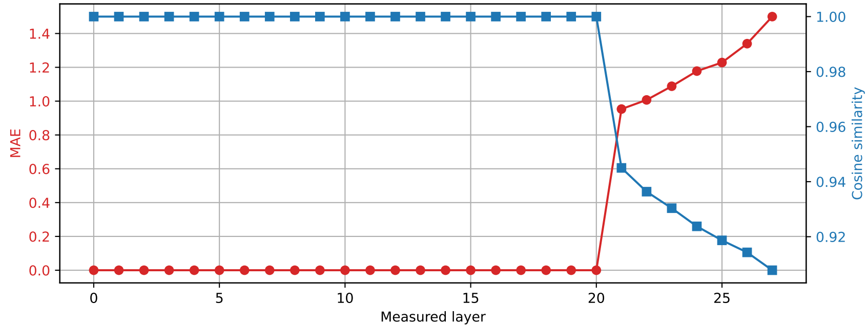
Qwen2.5-7B-Instruct | Prompt 0 Spared layer 20 | Hybrid vs quantized
