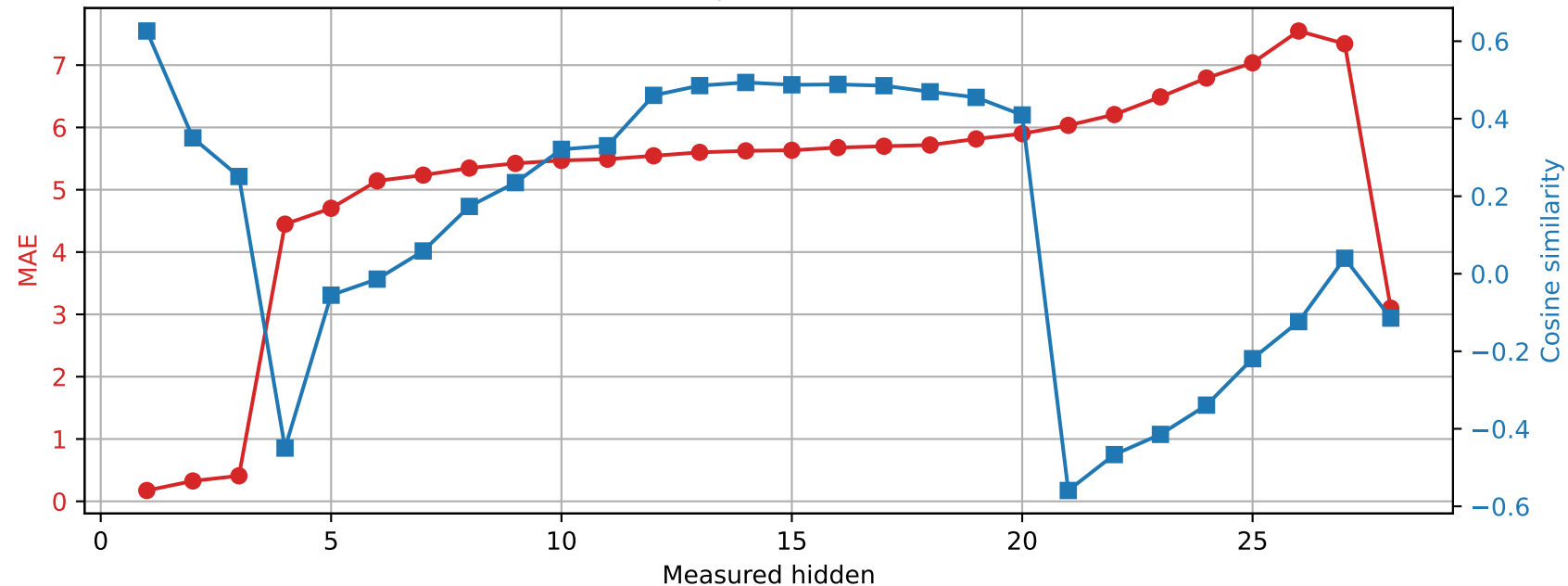
Qwen2.5-7B-Instruct | Prompt 0 Spared layer 27 | Unquantized vs hybrid
