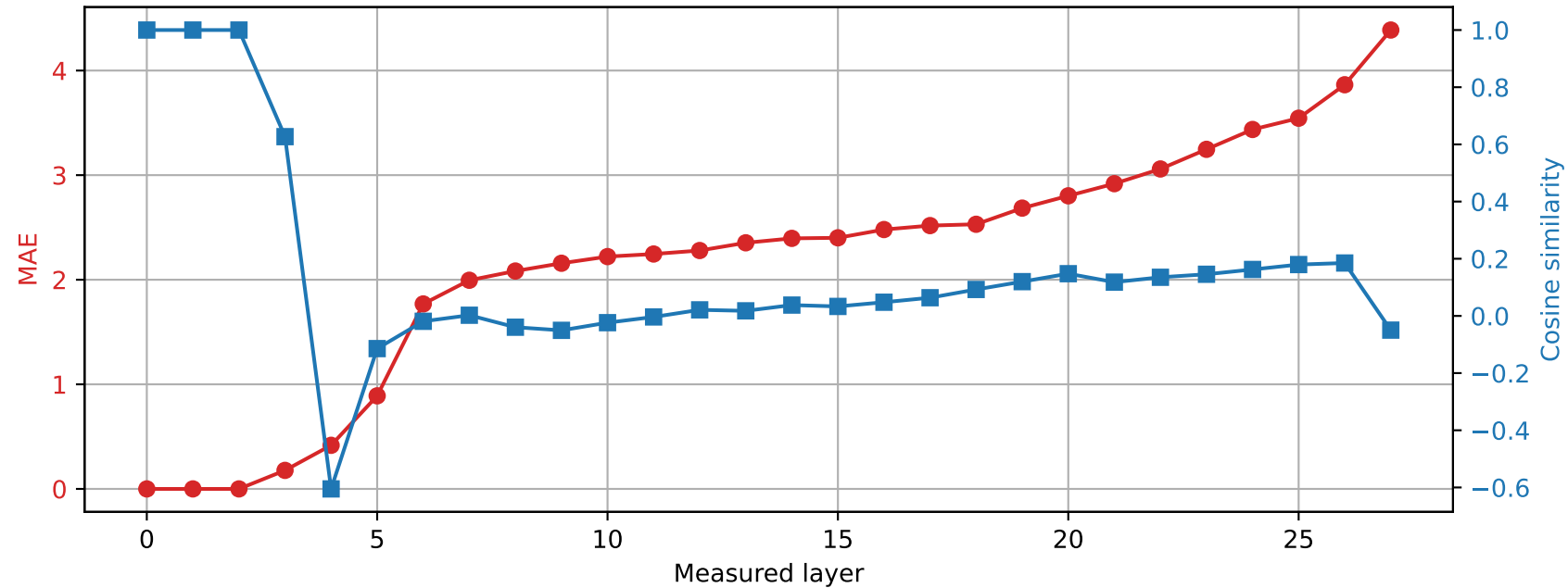
Qwen2.5-7B-Instruct | Prompt 1 Spared layer 2 | Hybrid vs quantized
