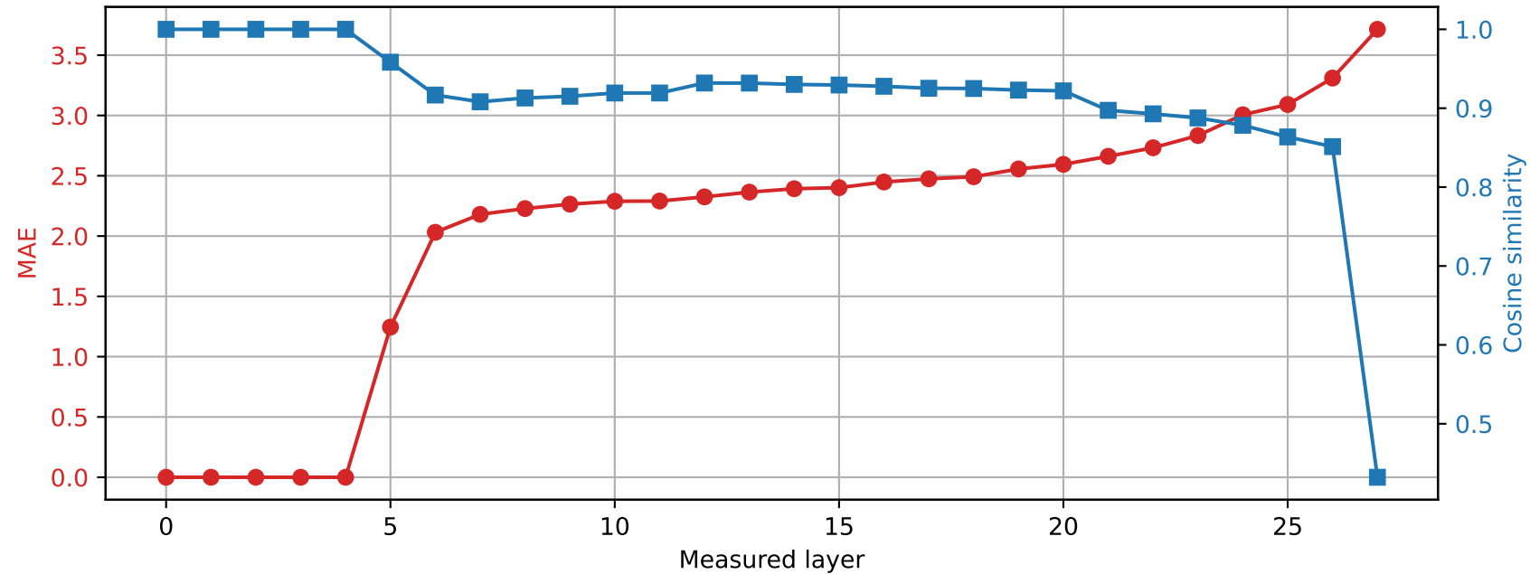
Qwen2.5-7B-Instruct | Prompt 1 Spared layer 4 | Hybrid vs quantized
