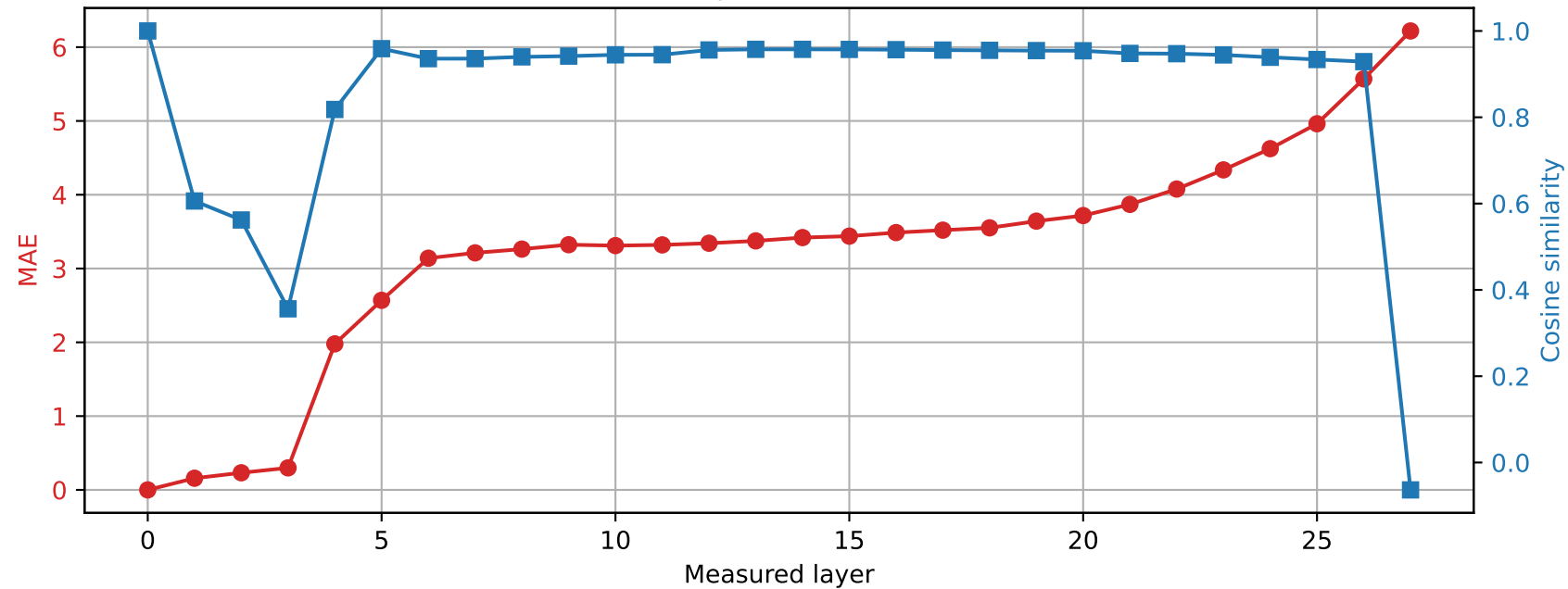
Qwen2.5-7B-Instruct | Prompt 1 Spared layer 4 | Hybrid vs unquantized
