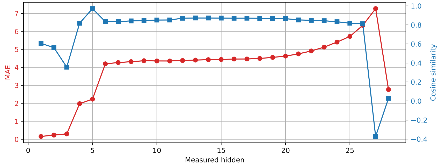
Qwen2.5-7B-Instruct | Prompt 1 Spared layer 5 | Unquantized vs hybrid
