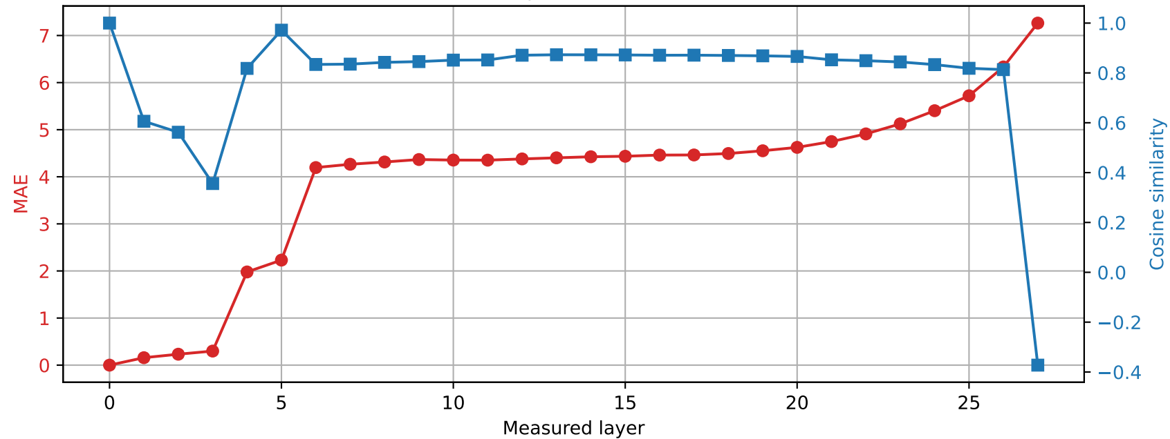
Qwen2.5-7B-Instruct | Prompt 1 Spared layer 5 | Hybrid vs unquantized
