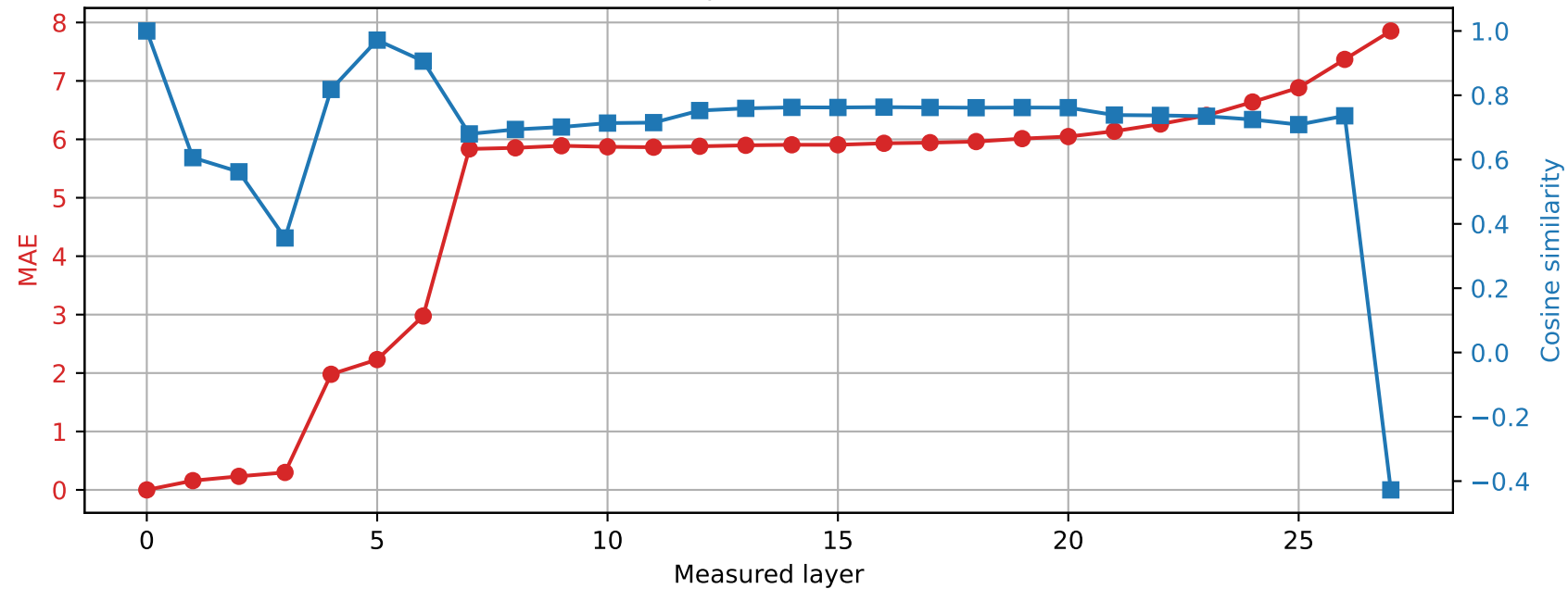
Qwen2.5-7B-Instruct | Prompt 1 Spared layer 6 | Hybrid vs unquantized
