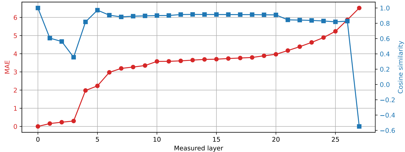
Qwen2.5-7B-Instruct | Prompt 1 Spared layer 9 | Hybrid vs unquantized
