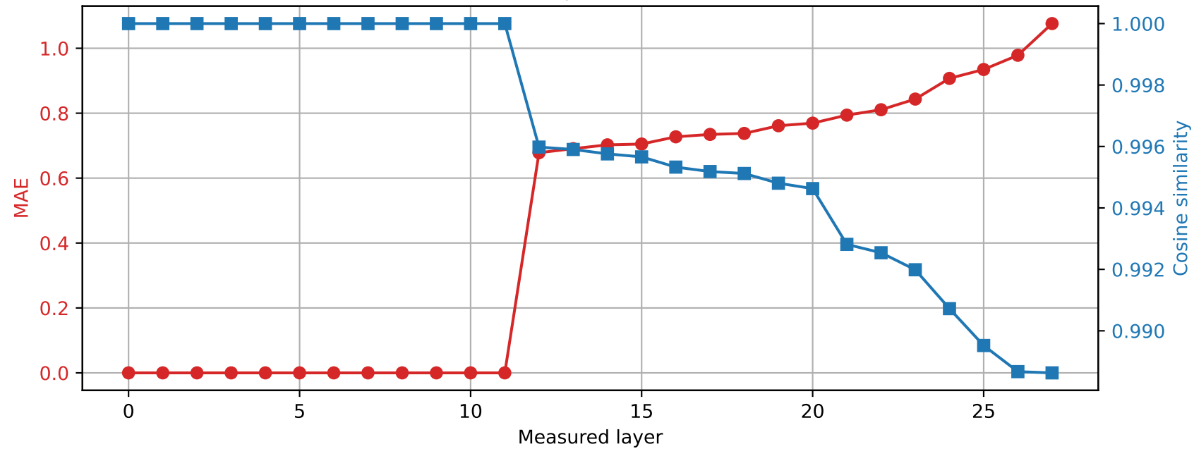
Qwen2.5-7B-Instruct | Prompt 1 Spared layer 11 | Hybrid vs quantized
