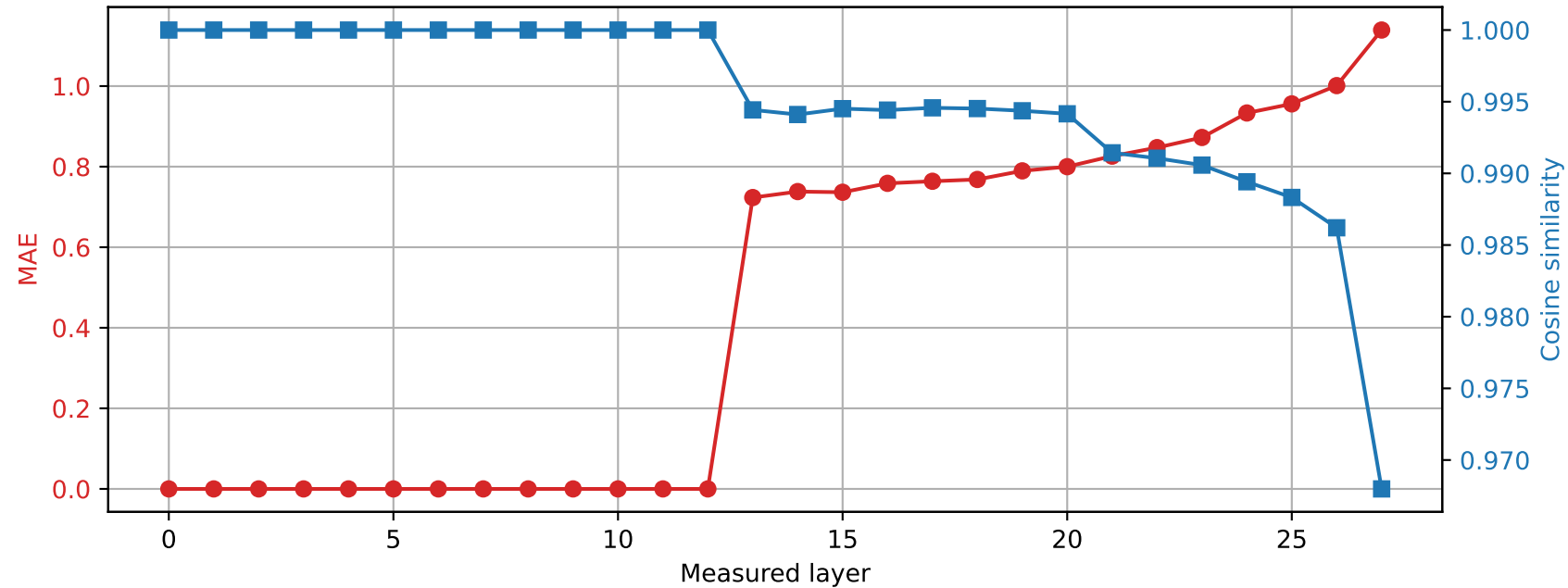
Qwen2.5-7B-Instruct | Prompt 1 Spared layer 12 | Hybrid vs quantized
