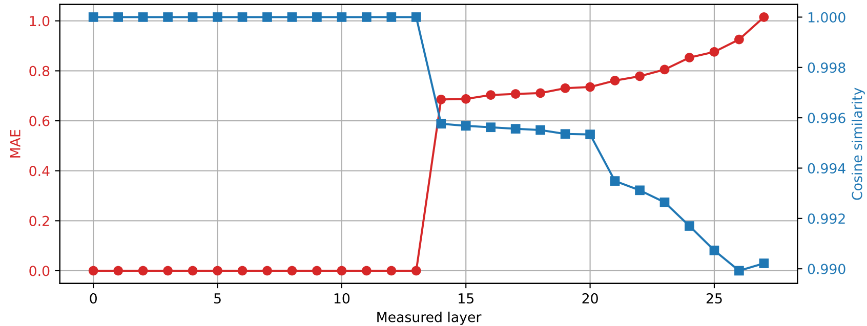
Qwen2.5-7B-Instruct | Prompt 1 Spared layer 13 | Hybrid vs quantized
